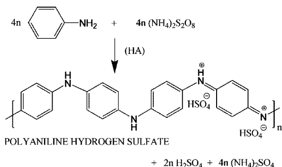
Scheme 3. Possible Reaction Involved in the Oxidation of Aniline with Ammonium Peroxydisulfate in the Presence of Alanine (HA) a
