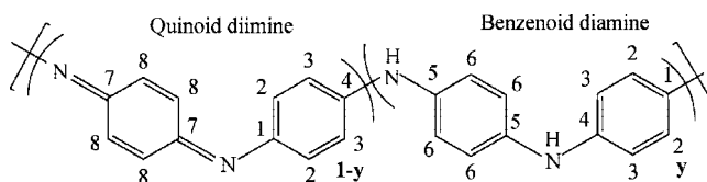
Scheme 1. Chemical Structure of Polyaniline
