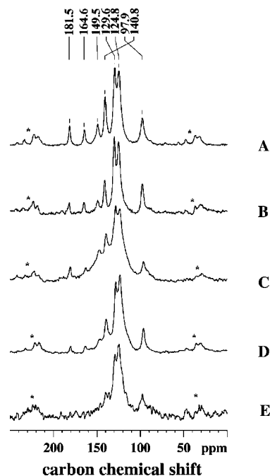
Figure 4. Solid-state 13 C CP/MAS NMR spectra of aniline oxidation products synthesized using APS in the presence of alanine: after 1 h reaction time (A), after 1 h reaction time and reduced with hydrazine (B), after 20 h reaction time (C), after 20 h reaction time and dedoped with NH 4 OH (D), and after 20 h reaction time and dedoped with LiOH (E). The asterisks denote spinning sidebands.
